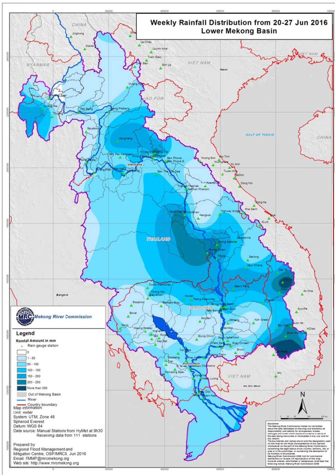
Figure 3: Weekly Rainfall Distribution over the LMB from 20 th – 27 th June, 2016
