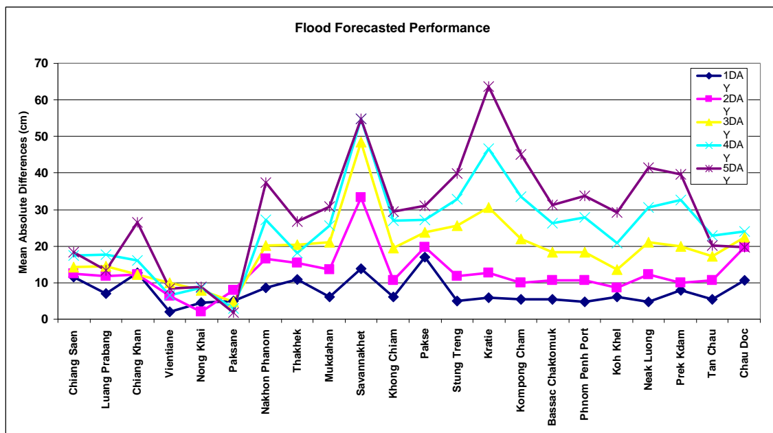
Figure B1: Average flood forecast accuracy along the Mekong mainstream (from 20 th – 27 th June 2016)
