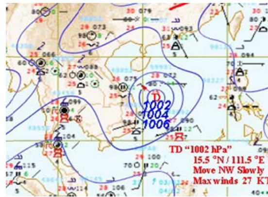
Figure 2: Weather map for 22 nd June 2016
