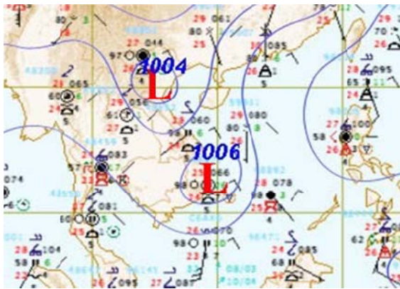
Figure 1: Weather map for 20 th June 2016
